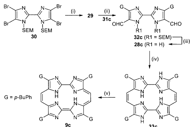
Scheme 3. Synthetic route for azaporphycenes 9 applied to 9c (G = p -BuPh): (i) BuLi/THF/–78 °C followed by DMF; (ii) p -butylphenylboronic acid ( 31c )/[Pd(PPh 3 ) 4 ]/Na 2 CO 3 /toluene/EtOH; (iii) HCl/EtOH/H 2 O; (iv) TiCl 4 /Zn(Cu)/THF; (v) O 2 in the presence of I 2
