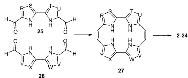
Scheme 1. Synthetic itinerary for azaporphycenes 2–24 showing the oxidized intermediate 27
