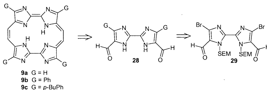
Scheme 2. Retrosynthetic analysis for 2,7,12,17-tetrasubstituted 3,6,13,16-tetraazaporphycenes 9
