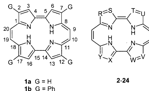
Figure 1. Porphycenes 1 and azaporphycenes 2–24 studied; R, S, T, U, V, W, X and Y are either CH or N (see text)
