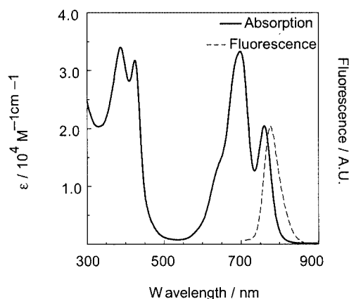
Figure 2. The UV/Vis absorption (—) and fluorescence (---) spectra of 9c ( G = p\text{-BuPh} )
